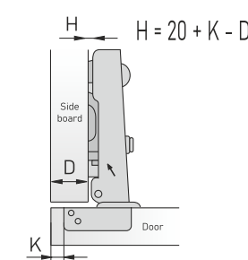
Full overlay C=0
