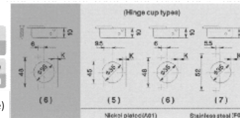
Series soft-close (snap-on, cam adjustable) hinges 110° with integrated damper
